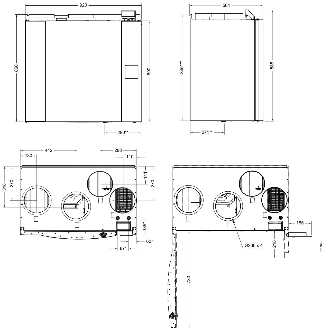
Pav. 3 Dimensions and weight, R model
